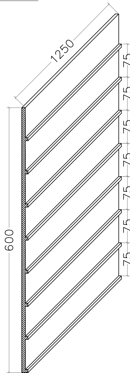
GRC CHANNEL (PANEL)
